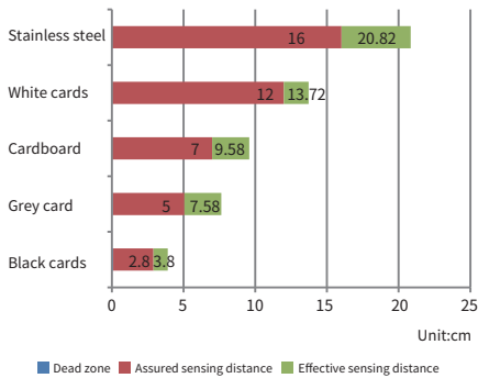
Diffuse reflection(PSV-BC**)
