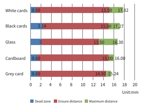
Background suppression(PSV-YR15**)
