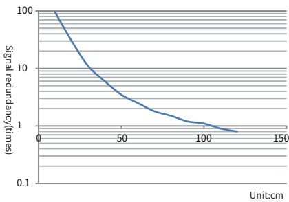
Through beam-Side light(PSV-TC**-S)
