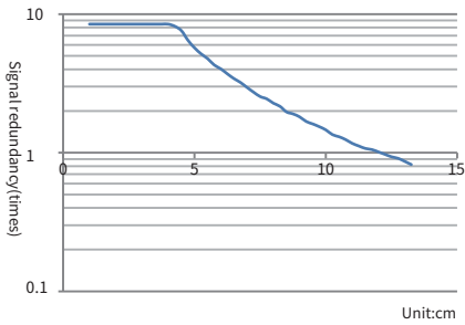
Diffuse reflection(PSV-BC**)
