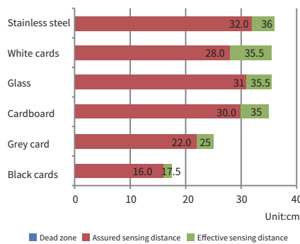
Convergent reflection(PSV-SR**)
