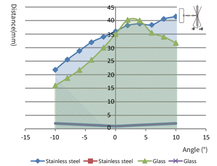
Convergent reflection(PSV-SR**)
